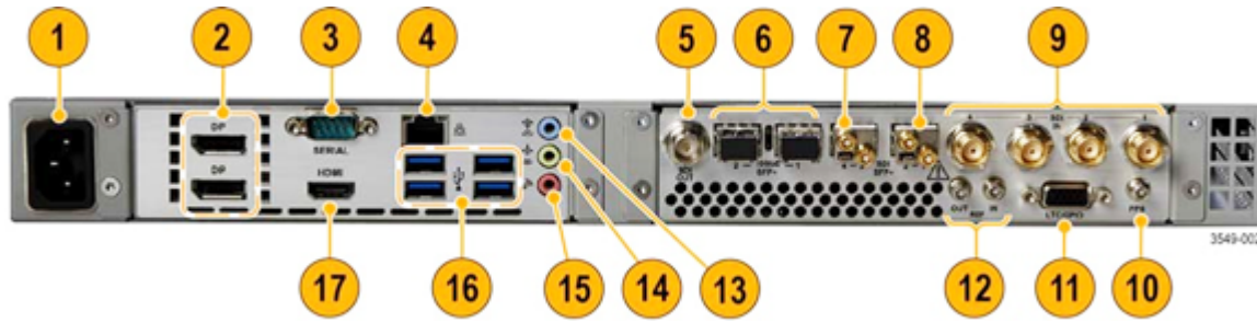
Descriptions of numbered PRISM MPX2-10 rear-panel connectors
