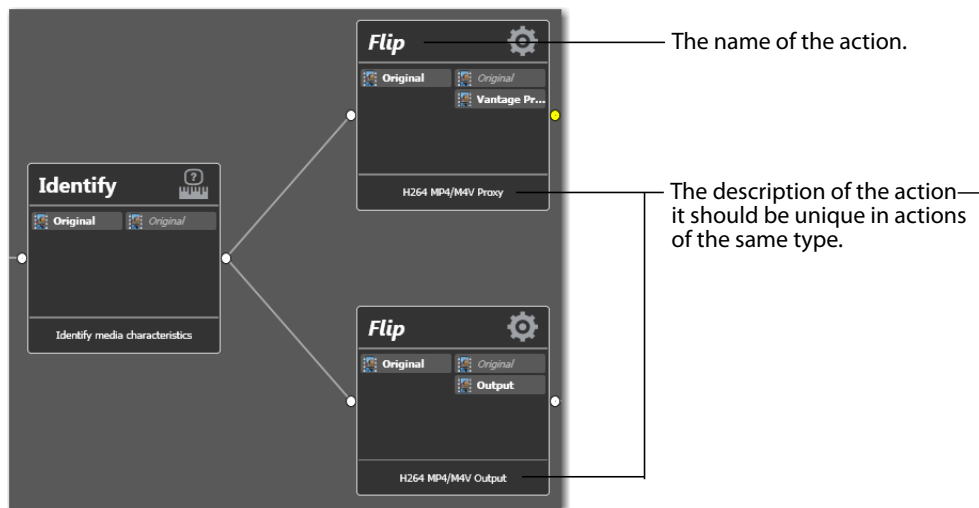
Figure 9. Identifying the Name and Description of Actions in a Workflow
