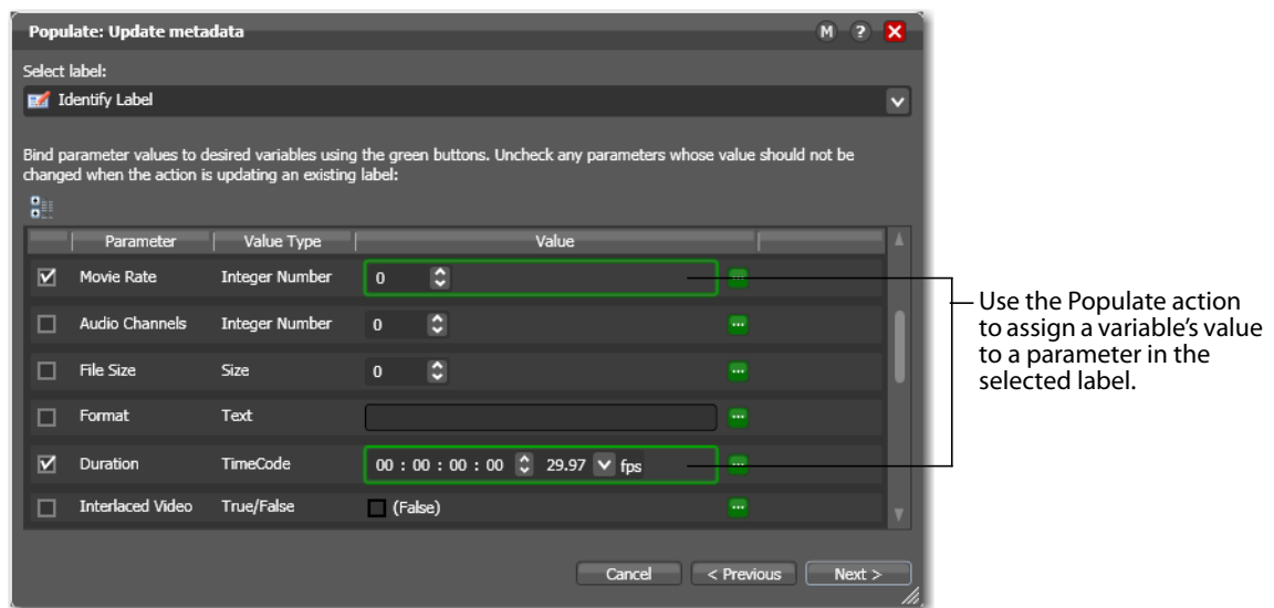
Figure 10. Binding Variables to Label Parameters in the Populate Action
