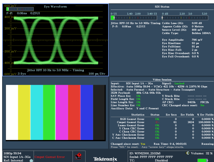
3G-SDI monitoring.
