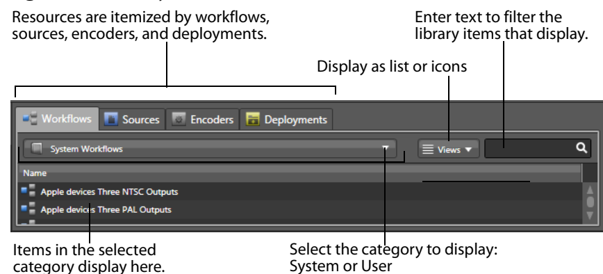
Figure 29. Library Panel
