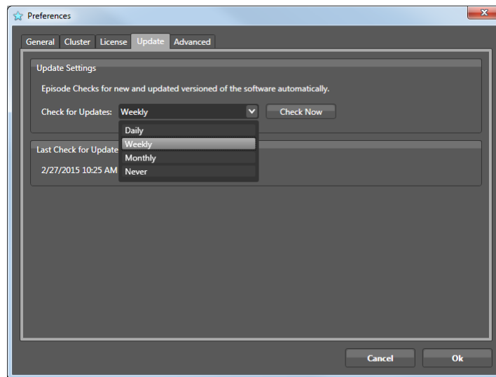
Figure 55. Preferences—Update Tab
