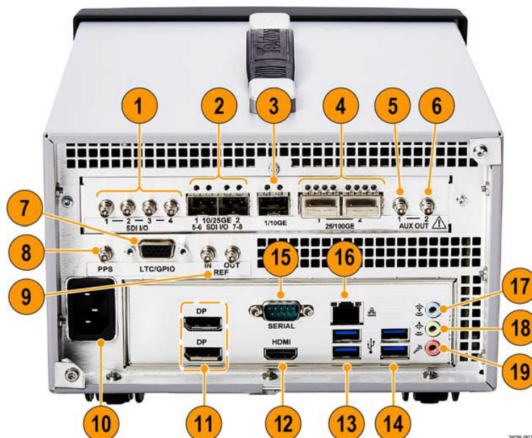
Descriptions of numbered PRISM MPI2-25 rear-panel connectors
