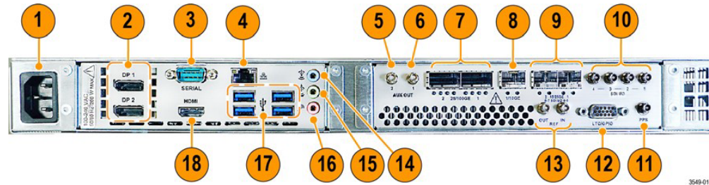
Descriptions of numbered PRISM MPX2-25 rear-panel connectors
