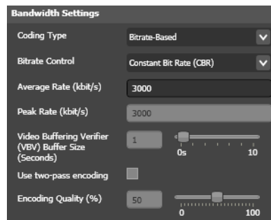
Figure 147. MPEG-2 Codec—Bandwidth Settings
