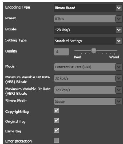
Figure 218. LAME MP3 Codec Settings
