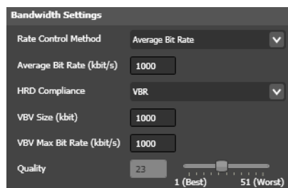
Figure 123. x264 Codec—Bandwidth Settings
