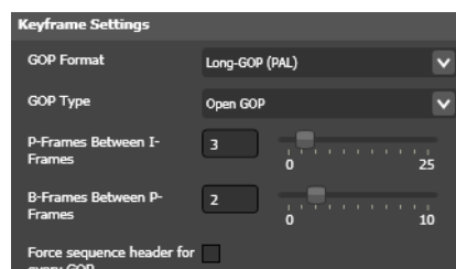
Figure 146. MPEG-1 Codec—Keyframe Settings
