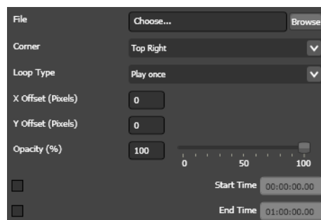
Figure 206. Watermark Filter Settings
