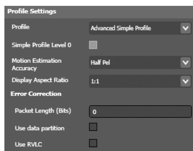
Figure 154. MPEG-4 codec—Profile Settings
