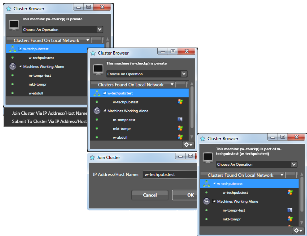
Figure 50. Cluster Browser Join by IP or Name (Submit is similar)
