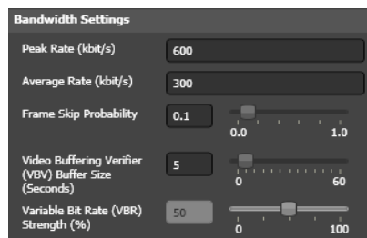
Figure 106. Flash 8 (VP6) Codec—Bandwidth Settings
