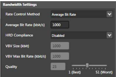
Figure 135. H.265 (x265)Codec—Bandwidth Settings
