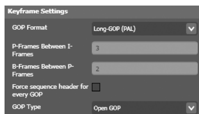
Figure 149. MPEG-2 Codec—Keyframe Settings
