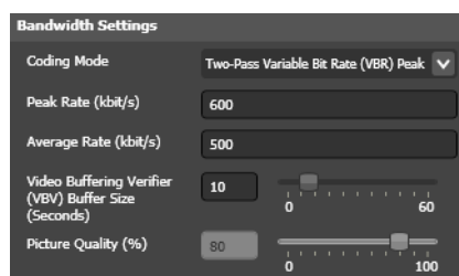
Figure 165. Windows Media Video 9 Codec—Bandwidth Settings
