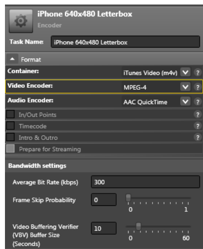
Figure 20. Inspector Panel for Encoders
