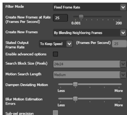
Figure 178. Advanced Frame Rate Filter Settings
