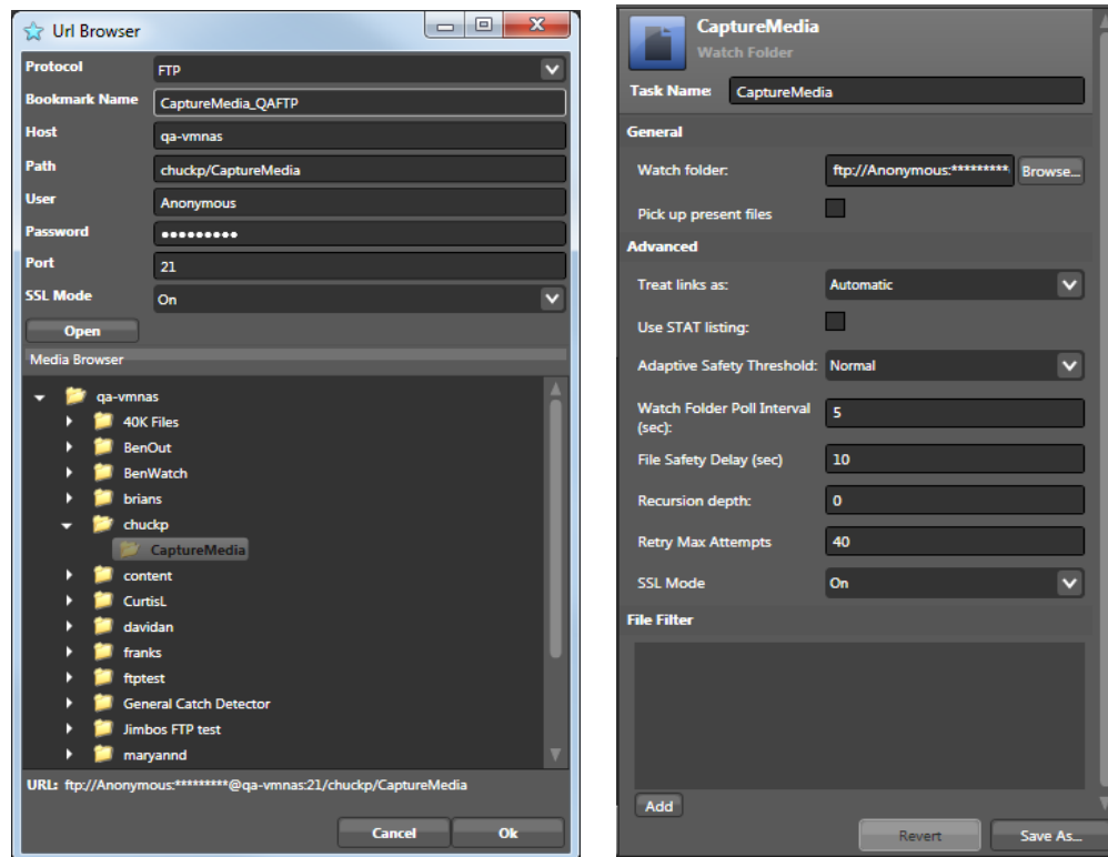
Figure 33. FTP/Network Share (SMB)/Wiretap Server Watch Folder Setup
