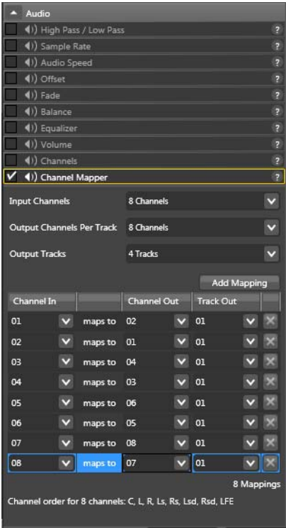
Figure 229. Channel Mapper Filter Settings
