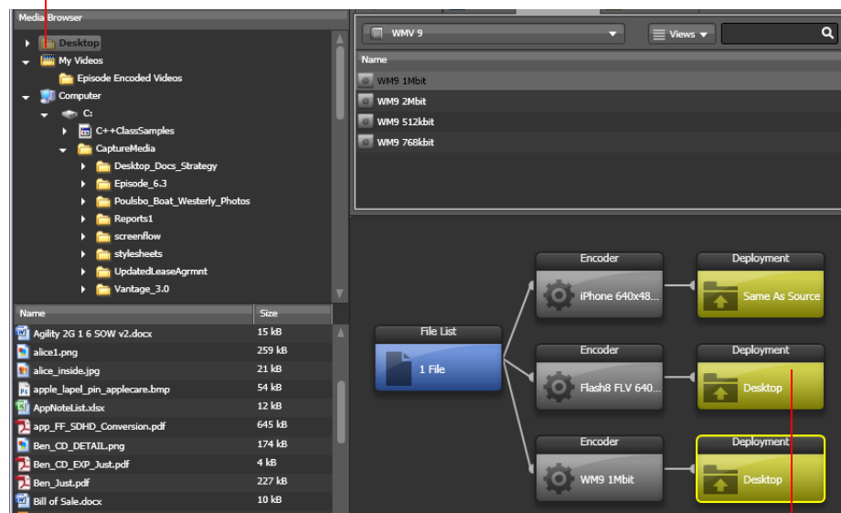
Figure 19. Adding Destinations to a Workflow
