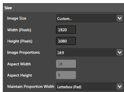
Figure 194. Resize Filter—Size Settings
