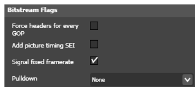
Figure 120. H264 Codec—Bitstream Flag Settings
