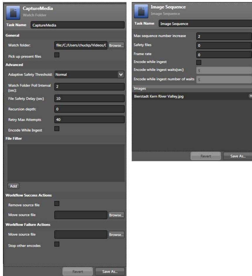
Figure 35. Source/Watch Folder and Image Sequence Inspector Panels
