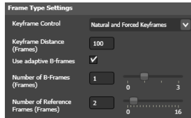
Figure 115. H264 Codec—Frame Type Settings
