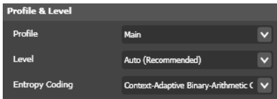
Figure 128. H264 Codec—Profile & Level Settings
