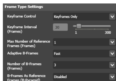
Figure 125. x264 Codec—Frame Type Settings
