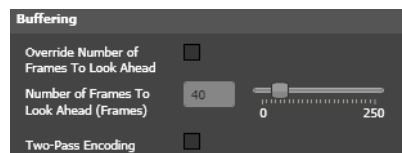
Figure 126. x264 Codec—Buffering Settings
