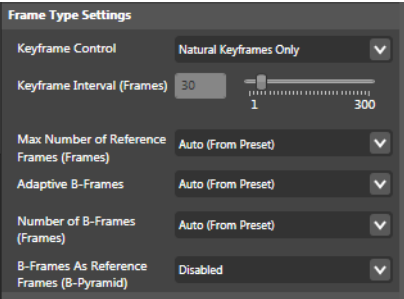
Figure 137. H.265 (x265) Codec—Frame Type Settings
