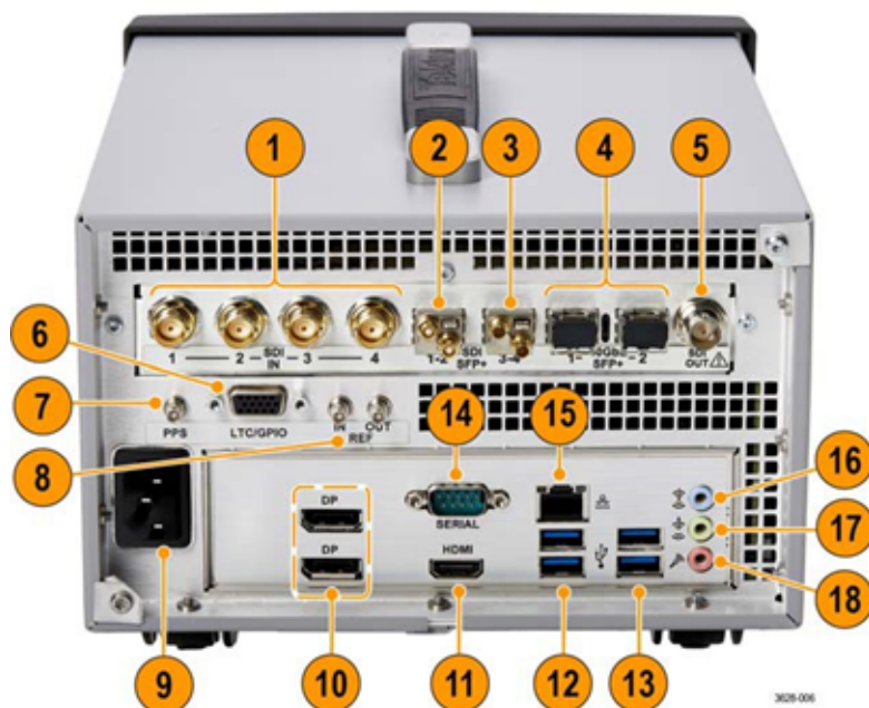
Descriptions of numbered PRISM MPI2-10 rear-panel connectors
