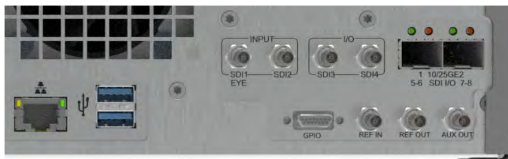
MPD-200/-300 Rear Panel Detail
